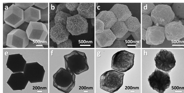
Figure 2. SEM and TEM images of a,e) ZIF-67, b,f) single-shelled ZIF-67@LDH, c,g) double-shelled CH@LDH nanocages, and d,h) CH@LDH/S.
